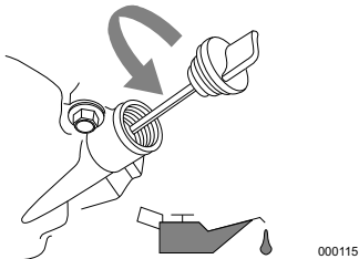
Figure 2-10. Remove Dipstick
