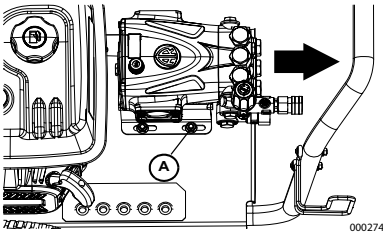
Figure 4-8. Pull Pump Away From Engine
